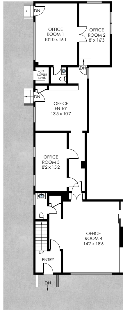
MAIN LEVEL 1300 FIN. SQ. FT. 9'9 CEILING
